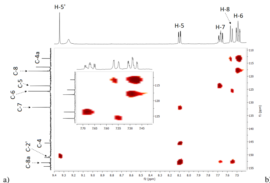
Figure 4. HMBC a) spectrum and b) correlations of compound (5).
