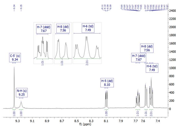
Figure 1. ^1\text{H} NMR ( \text{CDCl}_3 , 400 MHz) spectrum of compound (5).
