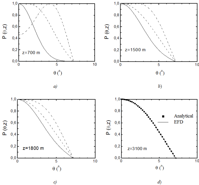
Figure 1. Normalized output angular power distribution obtained by EFD method at different locations along the CGW-CGE-68 fiber for three Gaussian input angles \theta_0 = 0^\circ (solid line), 3^\circ (dashed line) and 6^\circ (dotted line) at: (a) z = 700 \text{ m} ; (b) z = 1500 \text{ m} ; (c) z = 1800 \text{ m} and (d) z = 3100 \text{ m} . [Drljaca, 2011.].
