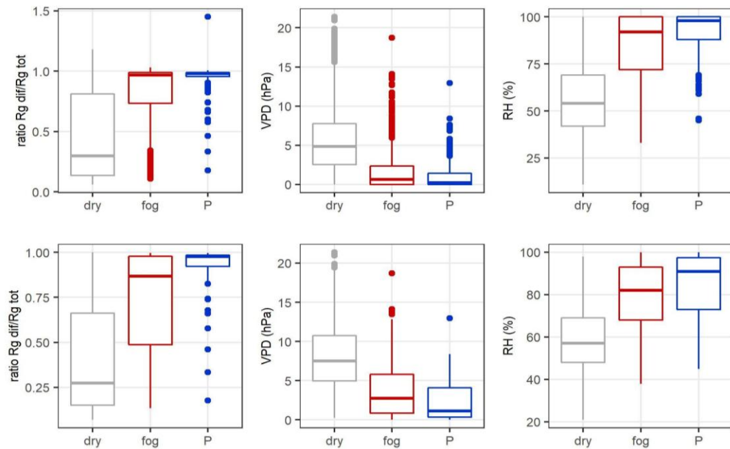
Figure 4. Weather conditions at times of fog (less than 1 km visibility), precipitation, and dry conditions (dry) from 01/01/2015 to 30/08/2015 (top row) and from 25/05/2015 to 30/08/2015 (bottom row) (ratio of diffuse to total global radiation, vapor pressure deficit VPD, and relative air humidity RH).
