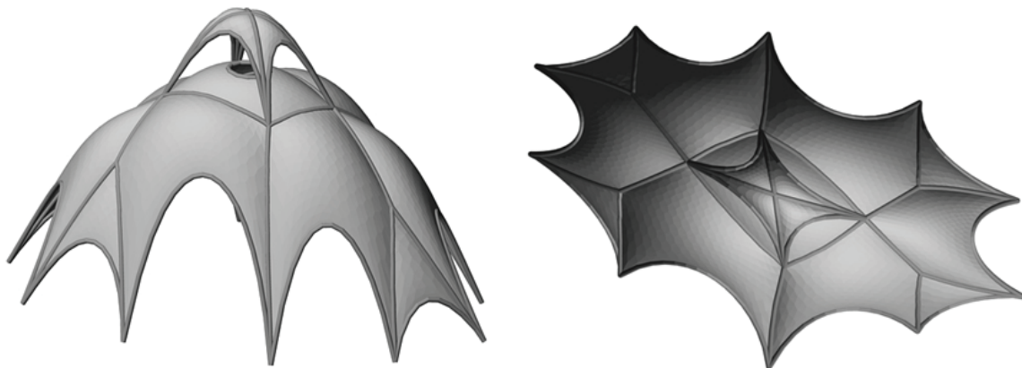
Figure 5: Two-storey compression structure computed using TM-FDM: general (left) and plan (right) views
