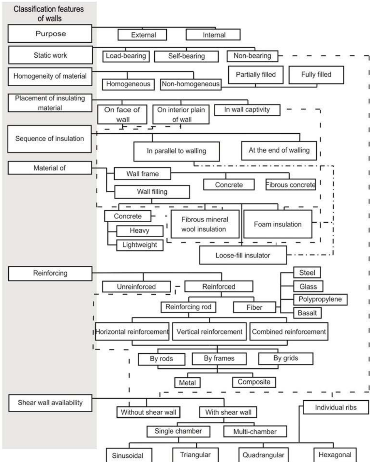
Figure 5: Classification of building walls erected using a 3D printer
