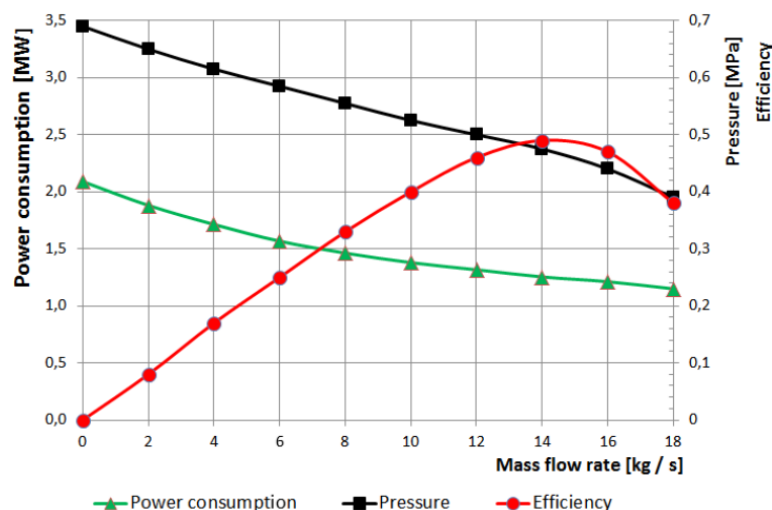
Figure 7: Theoretical characteristics of the experimental labyrinth compressor
