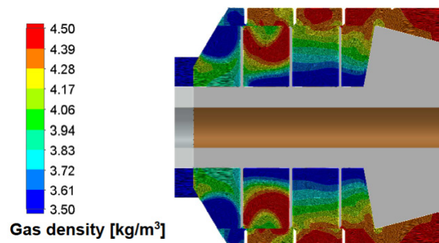
Figure 9: Change in gas density in the compressor flow section
