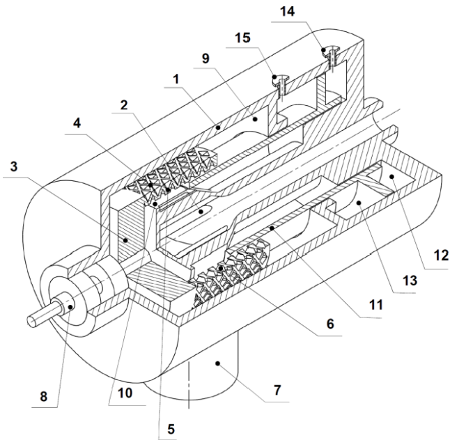
Figure 4: Scheme of the turbine with an open nozzle in isometric view
