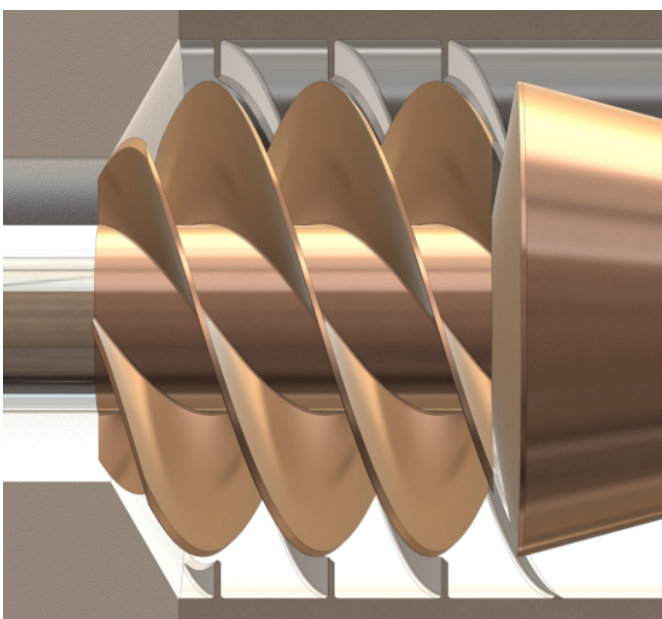
Figure 6: Three-dimensional model of the labyrinth compressor
