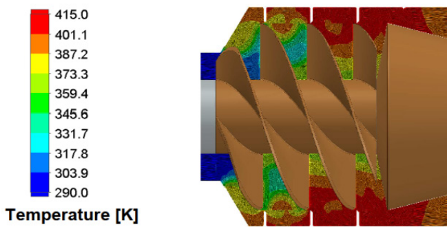
Figure 11: Change in gas temperature in the compressor flow section
