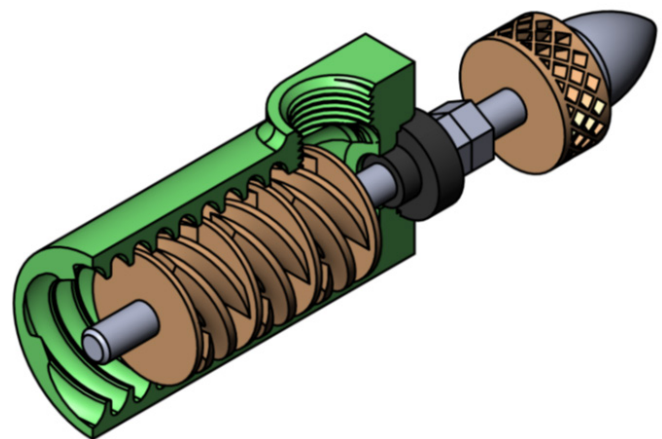
Figure 12: Three-dimensional computer model of the labyrinth compressor in which the screw auger is replaced with a set of vane wheels of axial type
