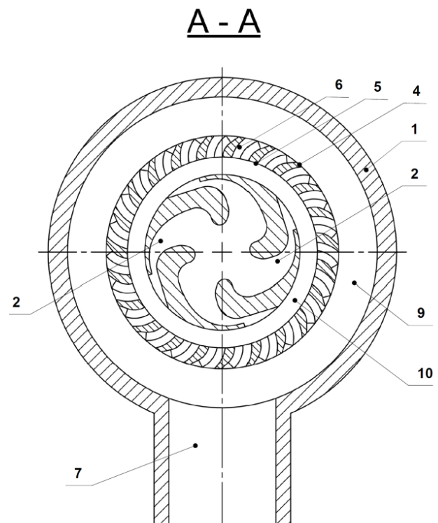
Figure 3: Cross section of the turbine
