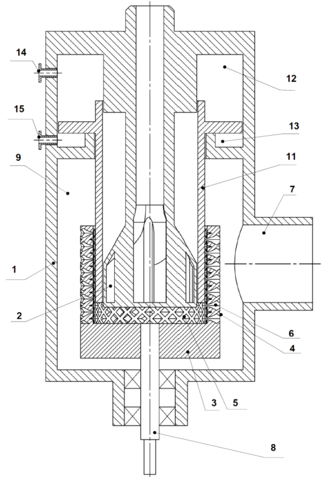
Figure 2: Scheme of the turbine with a closed nozzle
