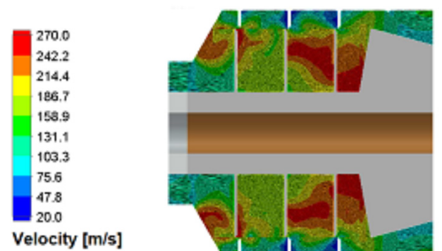
Figure 10: Change in gas velocity in the compressor flow section
