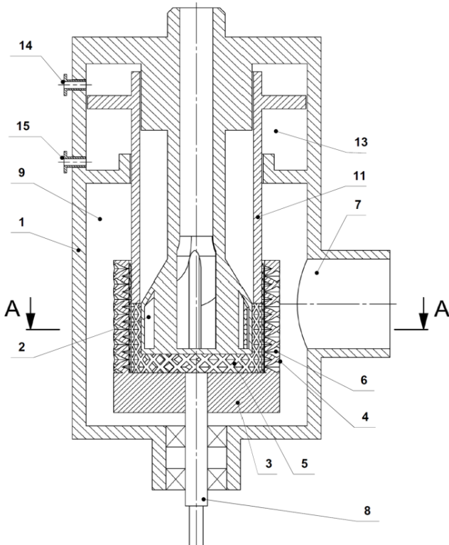
Figure 1: Scheme of the turbine with an open nozzle
