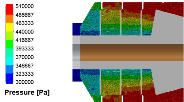
Figure 8: Change in gas output pressure in the compressor flow section
