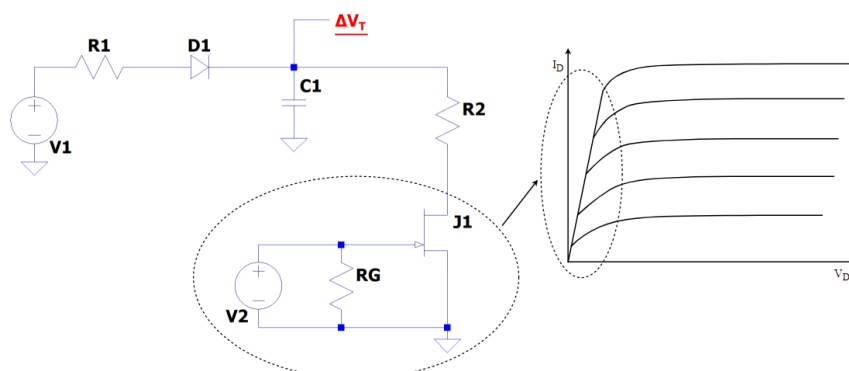
Figure 4: Electrical circuit for NBTI modeling
