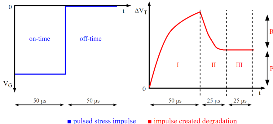
Figure 3: The waveform of stress voltage during the pulsed NBT stress and resulting micro-level signal of \Delta V_T ( R – recoverable component, P – permanent component)
