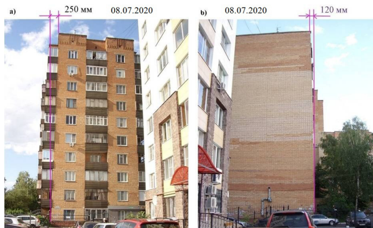
Figure 2: The size of the tilt: a) a residential building on Zelenko street (Kursk); b) a residential building on Mirnaya street (Kursk)
