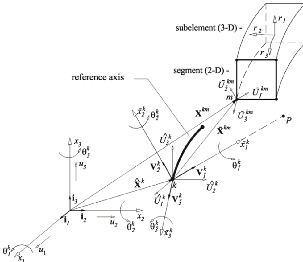
Figure 2: The geometry of the beam superelement with 2D cross-section seg-
