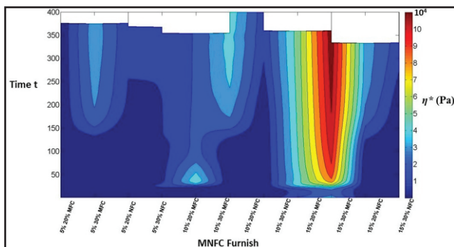
Figure 4: Increase in complex viscosity ( \eta^* ) as smoothed data rheogram for 5-15 wt-% consistency MNFC-containing furnishes in DSO mode
