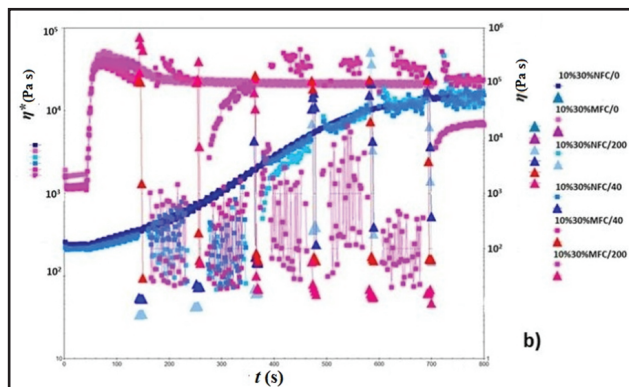
Figure 3: Apparent variation noise of rheological data at shear rate \dot{\gamma} = 0/40/200 \text{ s}^{-1} CSR dewatering for b) \eta^* and \eta for the 10 wt-% MNFC furnishes with data structure response variation immediately after application of vacuum
