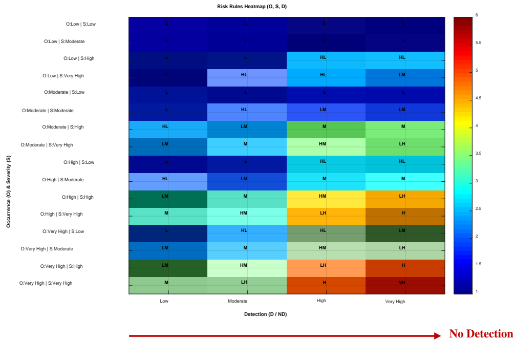
Fig. 3. Fuzzy FMECA Risk Rules based on O, S and D
