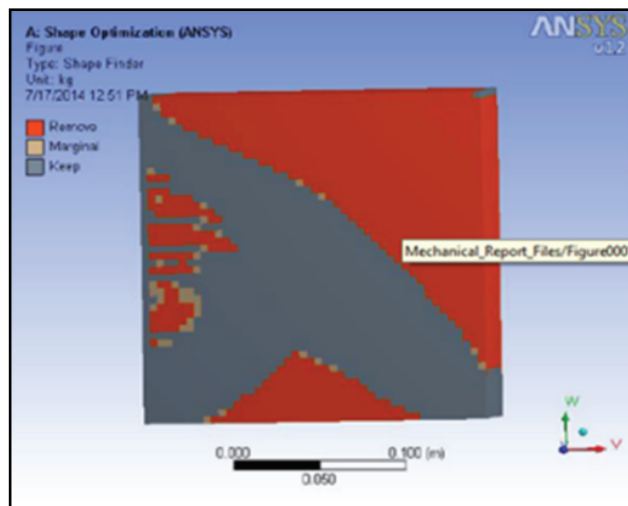
Figure 11: The converged solution after topological optimized domain
