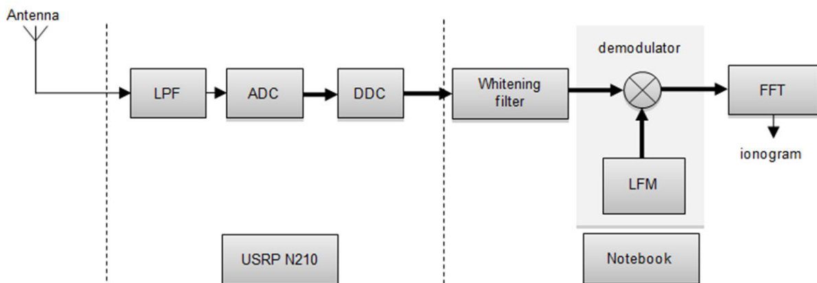
Figure 3: Block diagram of synthesis algorithms and processing continuous chirp signal
