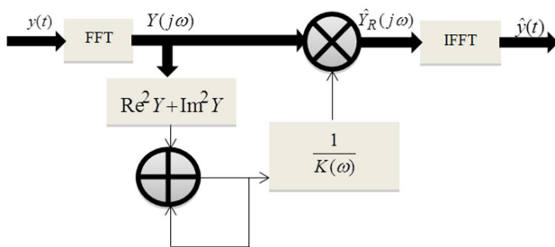
Figure 2: The algorithm of adaptive whitening interference on HF
