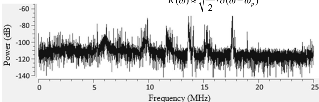
Figure 1: Instantaneous frequency spectrum of received power in the band of 25 MHz signals: continuous chirp, fluctuation noise and concentrated interference (vertical bars)
