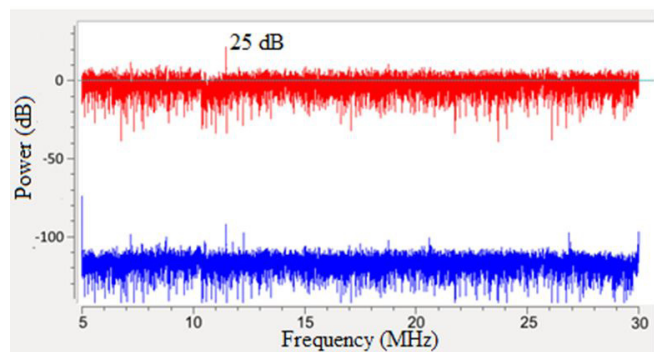
Figure 5: Results of whitening interference with chirp signal level less than 25 dB of the fluctuation noise.
