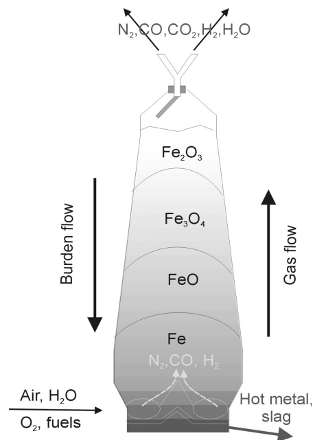
Figure 1. Blast furnace process with idealized locations of iron oxides
