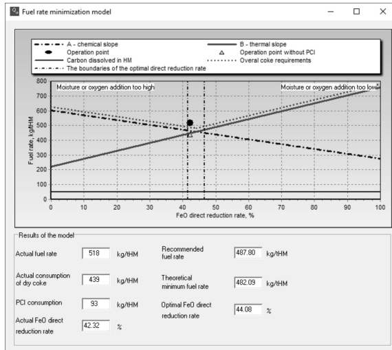
Figure 5. An example of the fuel rate minimization model working on real data
