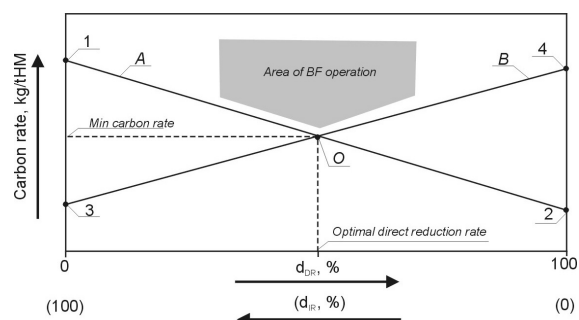
Figure 2. Carbon rate – FeO reduction ratio diagram for coke-only technology
