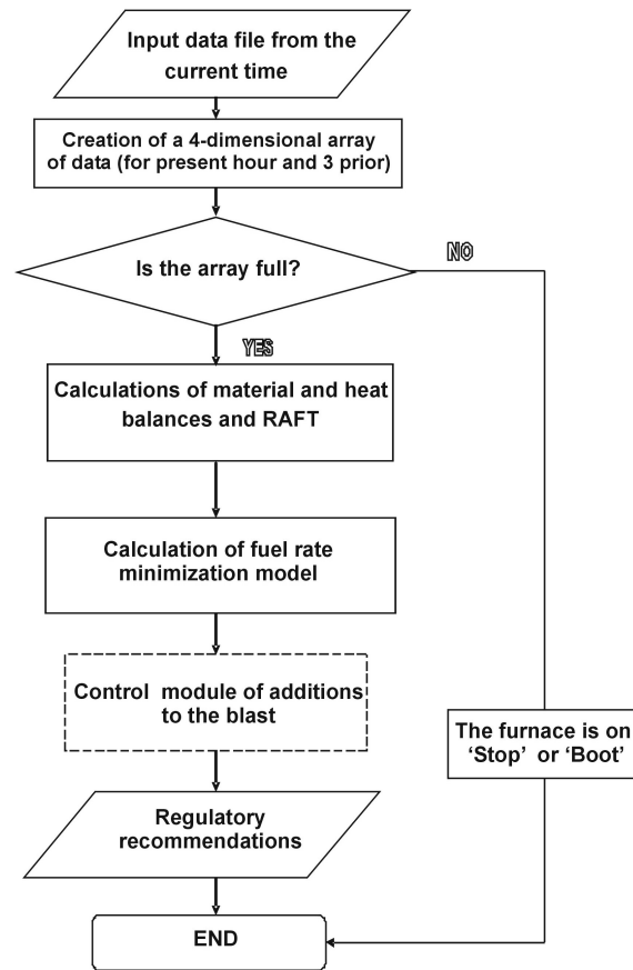
Figure 4. General schema of the parent algorithm
