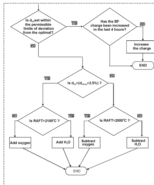
Figure 6. Control module of the blast parameter adjustments
