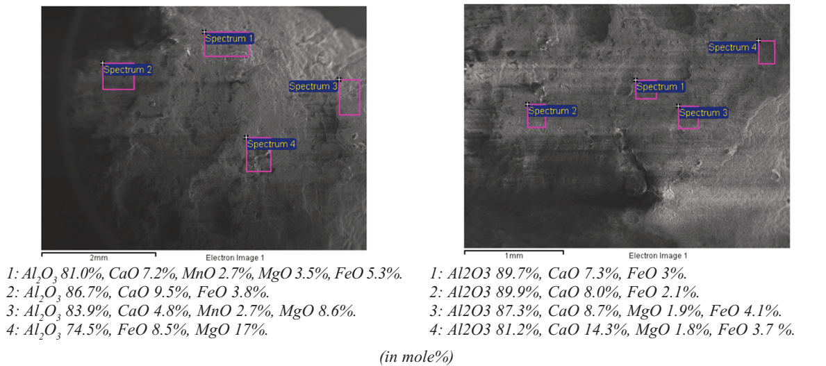
Figure 3. SEM-EDS analysis for the node
