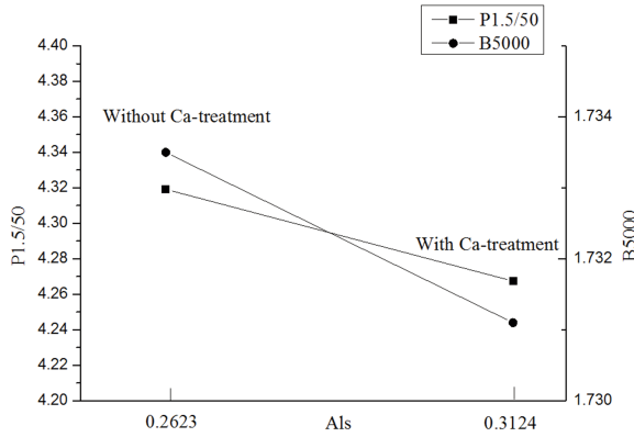
Figure 9. Magnetic properties and Als of the silicon steel with or without the addition of Ca, on average
