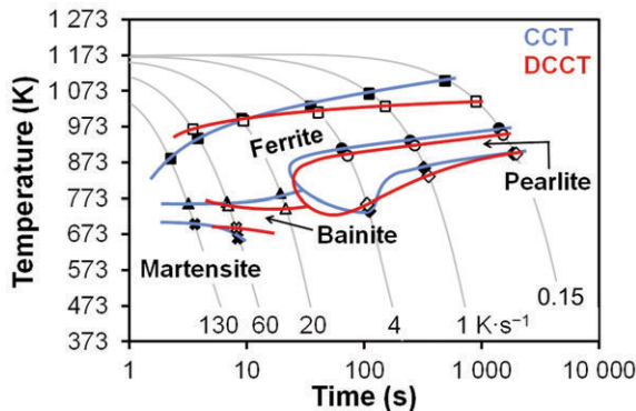
Figure 17. Superimposed CCT and DCCT diagrams, heating at 1173 K
