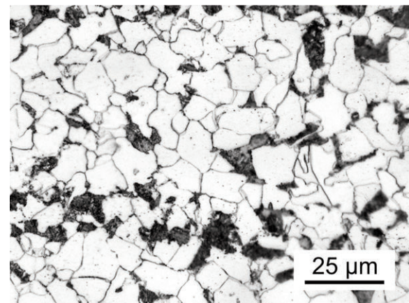
Figure 2. Fine-grained ferrite and pearlite microstructure after hot rolling and normalizing annealing
