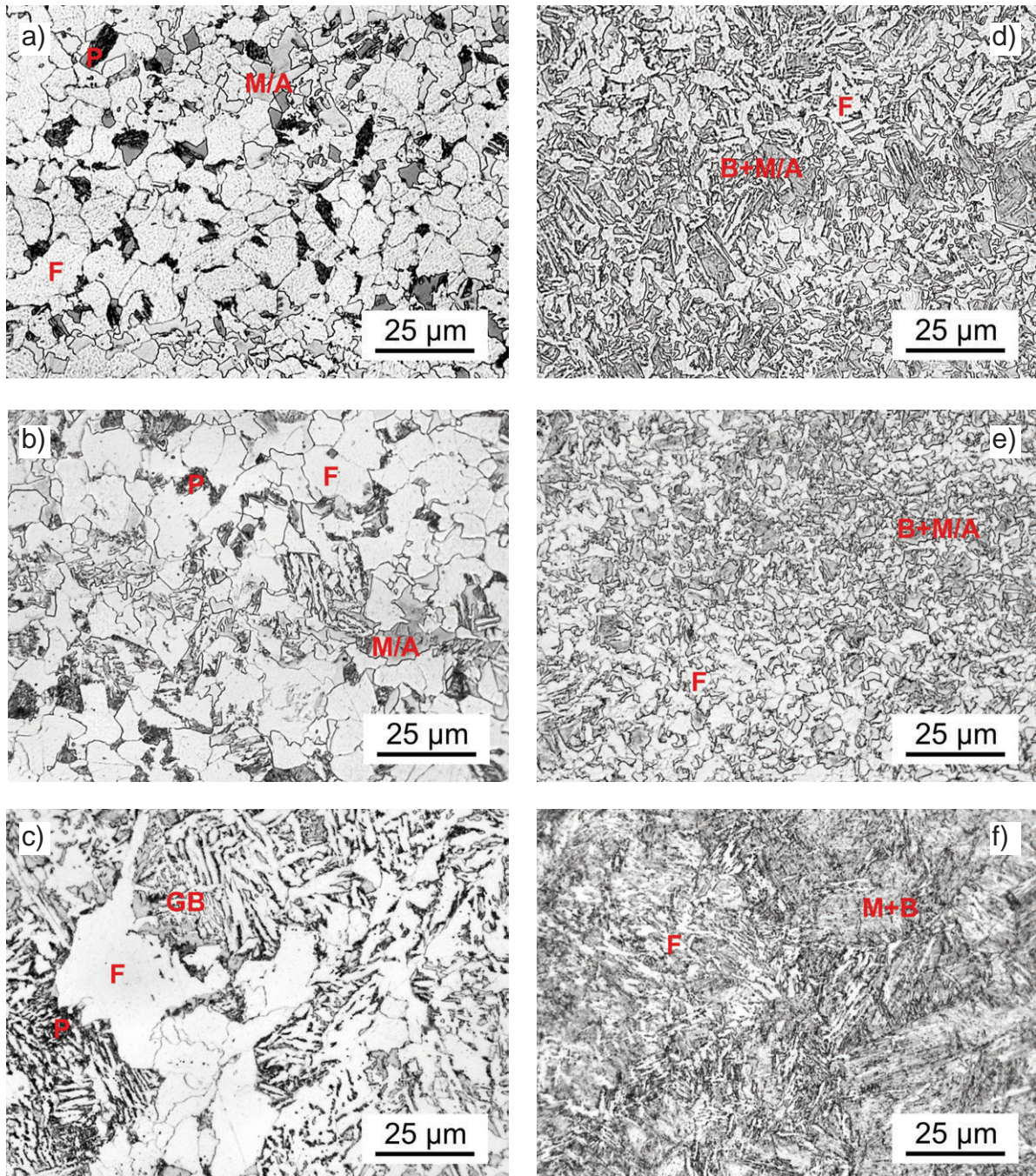
Figure 9. Comparison of typical microstructure of the dilatometer specimens a) CCT (heating at 1173 K, cooling 4 \text{ K}\cdot\text{s}^{-1} ); b) DCCT (heating at 1173 K, cooling 4 \text{ K}\cdot\text{s}^{-1} ); c) DCCT (heating at 1553 K, cooling 4 \text{ K}\cdot\text{s}^{-1} ); d) CCT (heating at 1173 K, cooling 35 \text{ K}\cdot\text{s}^{-1} ); e) DCCT (heating at 1173 K, cooling 35 \text{ K}\cdot\text{s}^{-1} ); f) DCCT (heating at 1553 K, cooling 35 \text{ K}\cdot\text{s}^{-1} )
