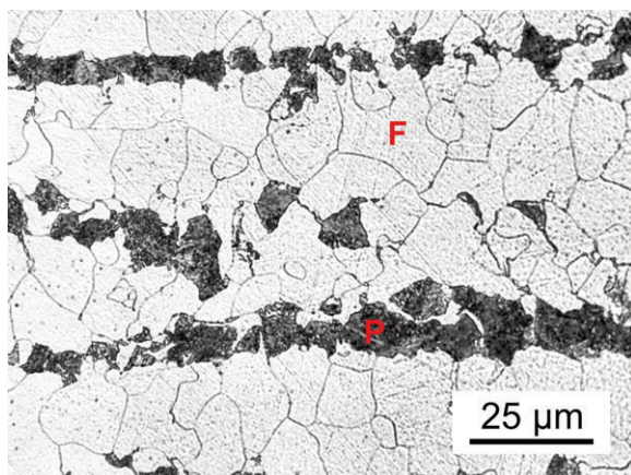
Figure 5. Banded ferrite and pearlite microstructure; CCT diagram – heating at 1173 K, cooling rate of 0.15 \text{ K}\cdot\text{s}^{-1}
