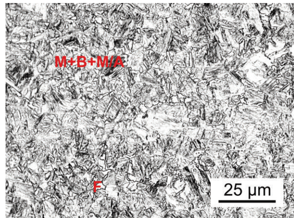
Figure 7. Microstructure formed by a mixture of martensite and bainite, the M/A component and a small fraction of polygonal ferrite; CCT diagram – heating at 1173 K, cooling rate of 180 \text{ K}\cdot\text{s}^{-1}
