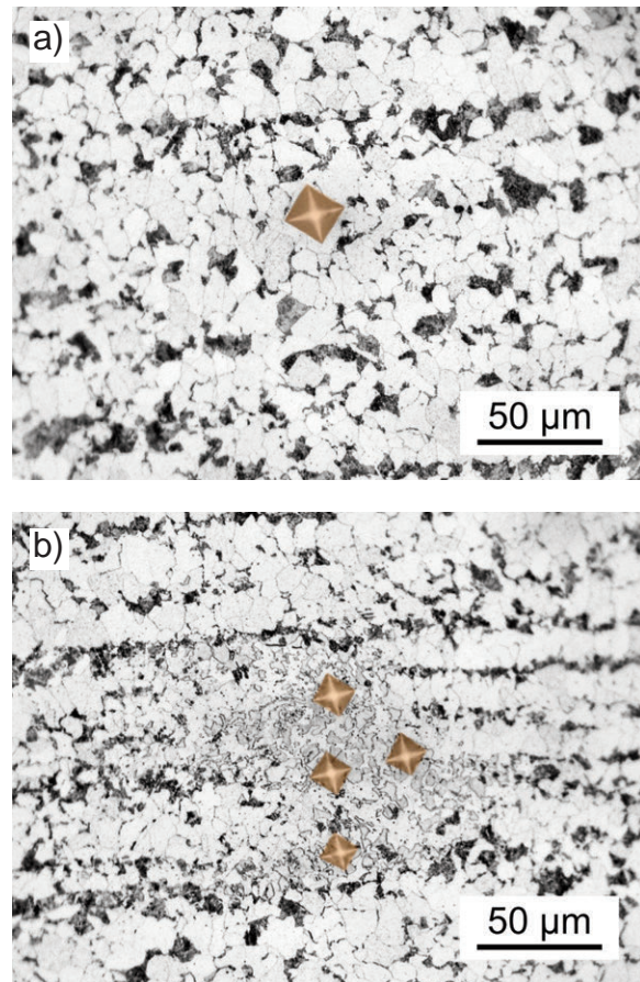
Figure 11. Local microstructure and microhardness heterogeneity after cooling at the rate of 1 \text{ K}\cdot\text{s}^{-1} – CCT diagram, heating at 1173 K a) ferrite and pearlite microstructure; the average microhardness of ferrite: \text{HV}_{0.05} = 153 ; b) an island of granular bainite containing M/A islands; the average microhardness of bainite: \text{HV}_{0.05} = 341
