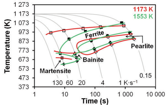
Figure 18. Superimposed DCCT diagrams – effect of the heating temperature 1173 K or 1553 K
