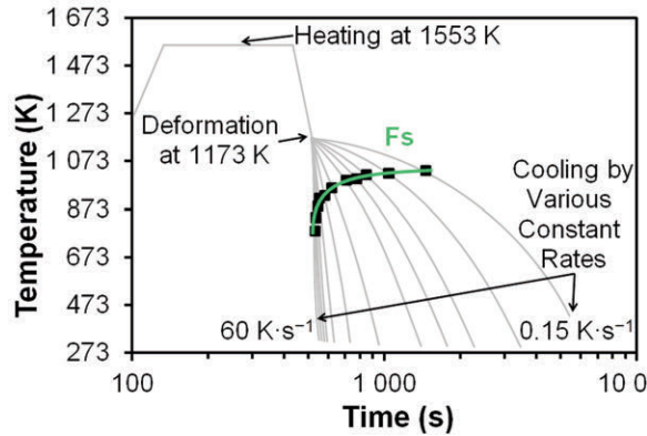
Figure 4. Scheme of the dilatometer tests after heating at 1553 K
