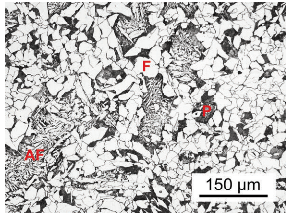
Figure 6. Microstructure formed by a mixture of equiaxed ferrite, pearlite and acicular ferrite; DCCT diagram – heating at 1553 K, cooling rate of 0.7 \text{ K}\cdot\text{s}^{-1}
