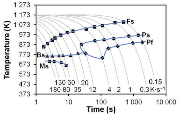
Figure 14. CCT diagram, heating at 1173 K
