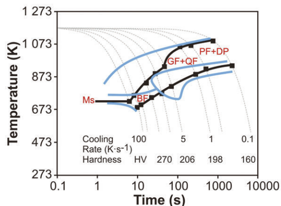
Figure 20. CCT diagram of the 28NbHC steel grade; black points and curves [6] superimposed with the CCT diagram presented in Fig. 14 – blue curves
