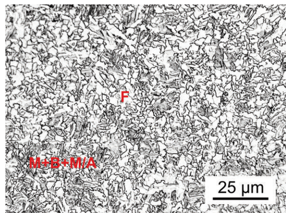
Figure 8. Microstructure consisting of a mixture of martensite and bainite, the M/A component and polygonal ferrite; DCCT diagram – heating at 1173 K, cooling rate of 80 \text{ K}\cdot\text{s}^{-1}
