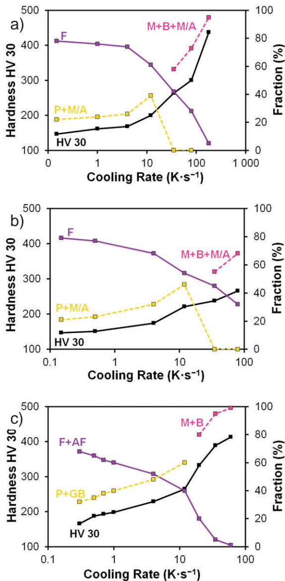
Figure 10. Dependence of hardness HV 30 and fractions of austenite decomposition products on the cooling rate a) CCT diagram – heating at 1173 K; b) DCCT diagram – heating at 1173 K; c) DCCT diagram – heating at 1553 K
