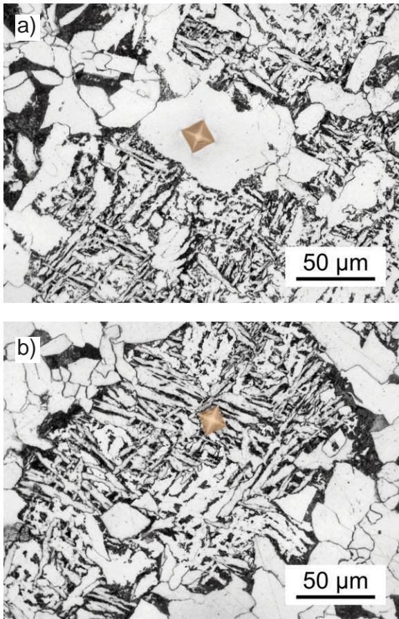
Figure 12. Microhardness of allotriomorphic ferrite and acicular ferrite + pearlite; DCCT diagram – heating at 1553 K, cooling rate of 0.7 \text{ K}\cdot\text{s}^{-1} a) polygonal ferrite, \text{HV}_{0.05} = 201 ; b) acicular ferrite and pearlite, \text{HV}_{0.05} = 267
