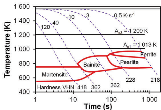
Figure 19. CCT diagram of a Nb-microalloyed steel constructed on the basis of combination of dilatometer and HAZ tests – according to [7]
