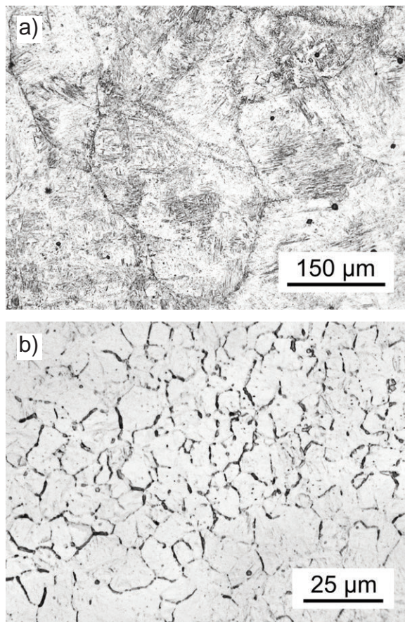
Figure 3. Effect of the heating temperature on the prior austenite grain size a) 1553 K b) 1173 K
