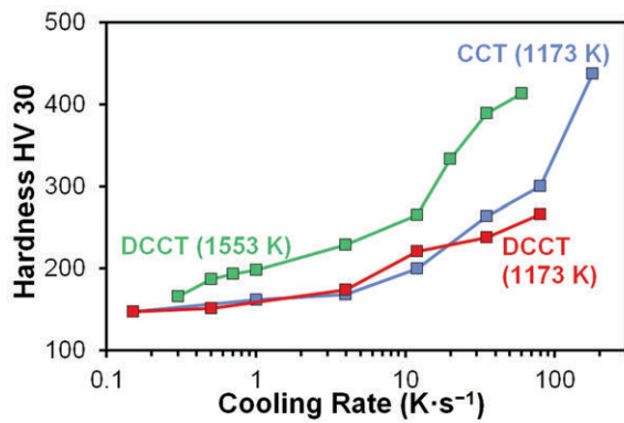
Figure 13. Effect of cooling rates and previous processing conditions on the hardness HV 30 of dilatometer specimens
