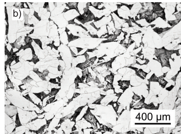
Figure 1. Microstructure of the bloom in the area of columnar crystals a) columnar crystals, polished state; b) coarse grained microstructure formed by a mixture of ferrite and pearlite
