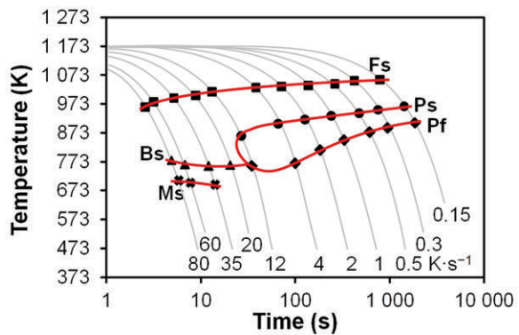
Figure 15. DCCT diagram, heating at 1173 K
