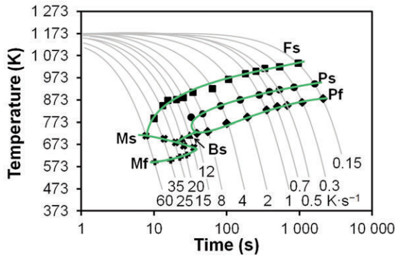
Figure 16. DCCT diagram, heating at 1553 K
