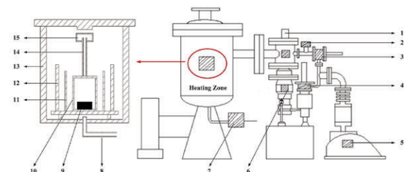
Figure 3. Schematic model of the vacuum distillation furnace 1. High vacuum valve; 2. Release valve; 3. Bypass valve; 4. Main valve; 5. Rotary vane pump; 6. Diffusion pump; 7. Inflation valve; 8. Vacuum pipe; 9. Raw materials; 10. Graphite crucible; 11. Graphite heater; 12. Heat shield; 13. Water cooled walls; 14. Graphite condensing pipe; 15. Condensation
