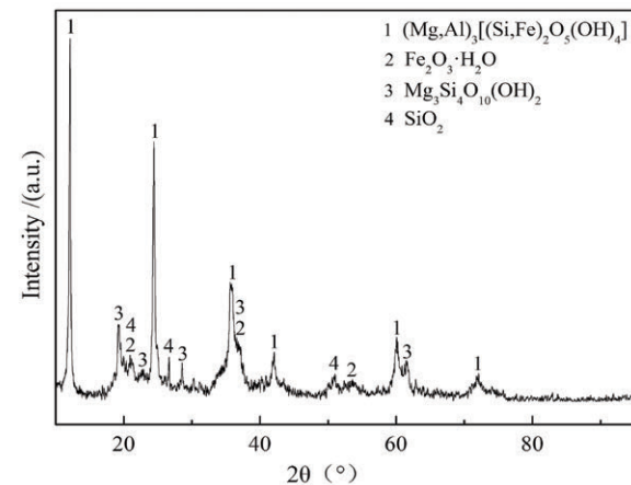
Figure 2. XRD patterns of garnierite
