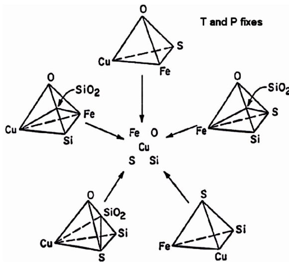
Figure 1. Quinary system Cu-Fe-S-O-SiO 2 , T and P fixes.
