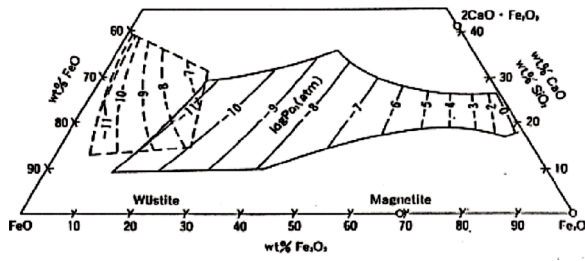
Figure 3. Isotherm at 1300 °C and isobars of oxygen potentials for ternary systems FeO-Fe 2 O 3 -SiO 2 and FeO-Fe 2 O 3 -CaO.
