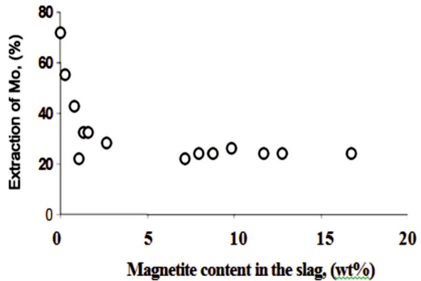
Figure 8. Extraction of molybdenum related to magnetite content.
