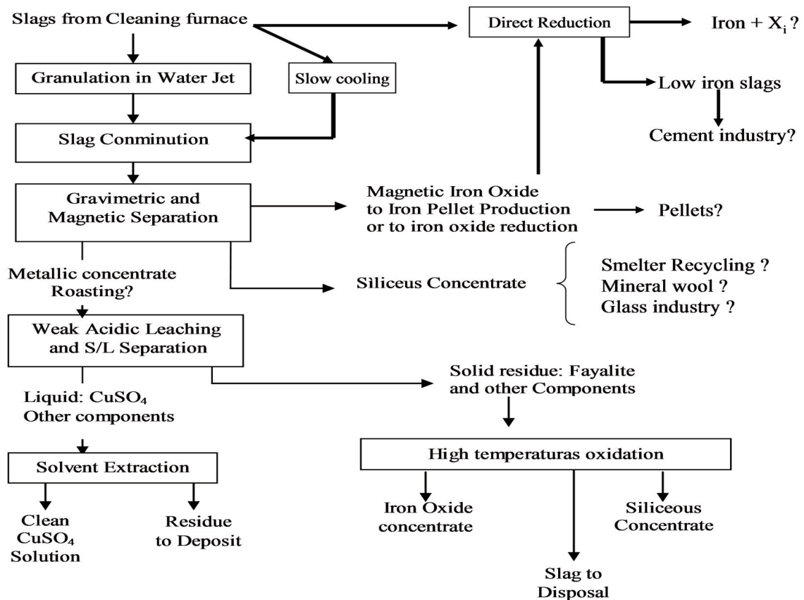
Figure 11. Flowsheet proposed for metal/material extraction from non ferrous slags.
