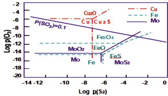
Figure 5. Stability diagram for copper and molybdenum in Cu-Mo-Fe system, 1300°C.
