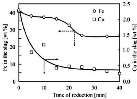
Figure 9. Concentration of copper and iron as function of time.
