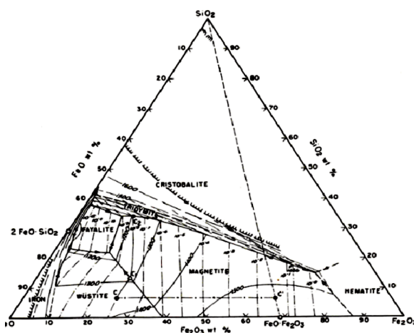
Figure 2. \text{FeO-Fe}_2\text{O}_3\text{-SiO}_2 ternary system.
