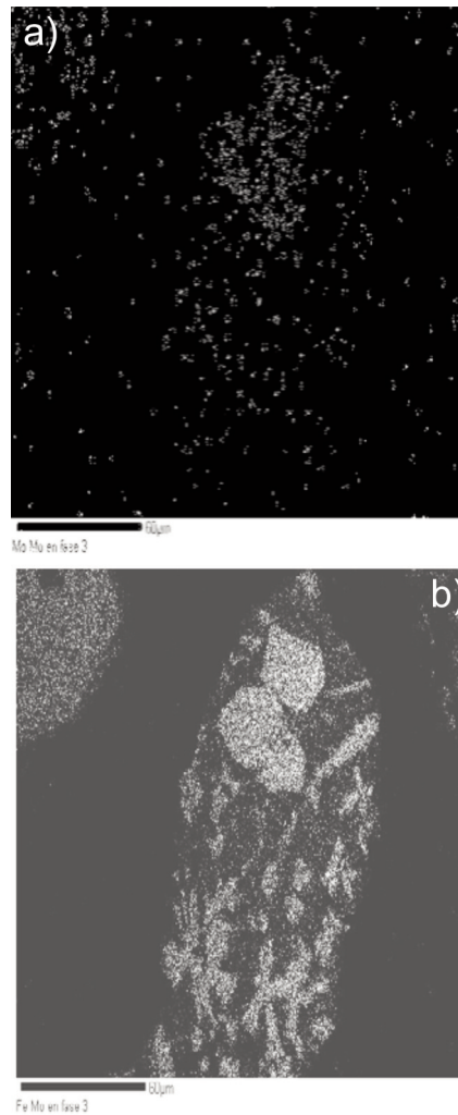
Figure 6. SEM analysis for molybdenum (a) and iron (b) distribution in slag.
