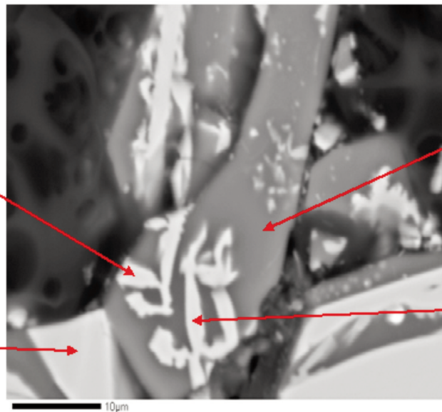
Figure 7. SEM characterization of a copper slag.
