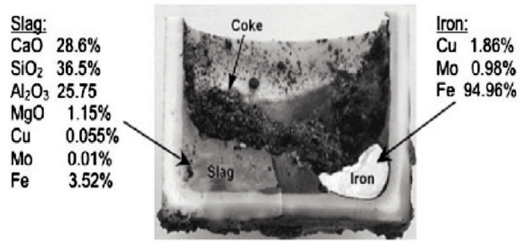
Figure 10. Slag and iron-rich alloy obtained at 1460°C in an alumina crucible.
