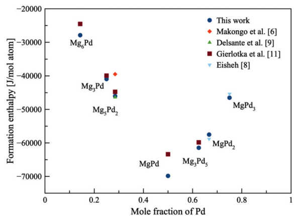
Figure 4. Formation energies of intermediate phases in the Mg-Pd system
