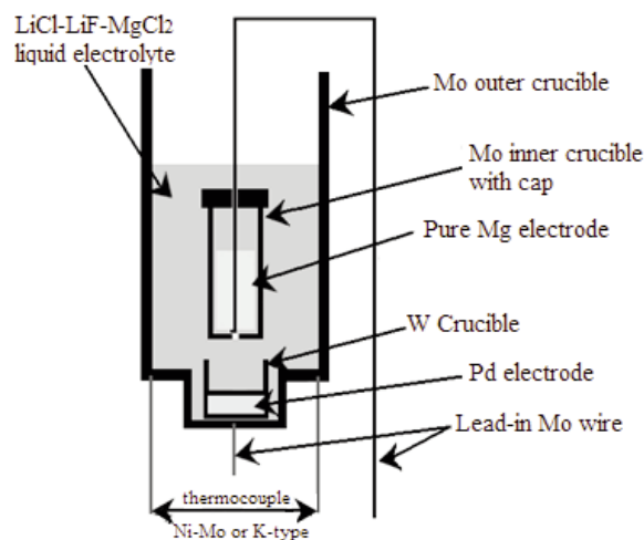
Figure 2. Scheme of the measuring cell used in the study of the electromotive force of alloys from the Mg-Pd system
