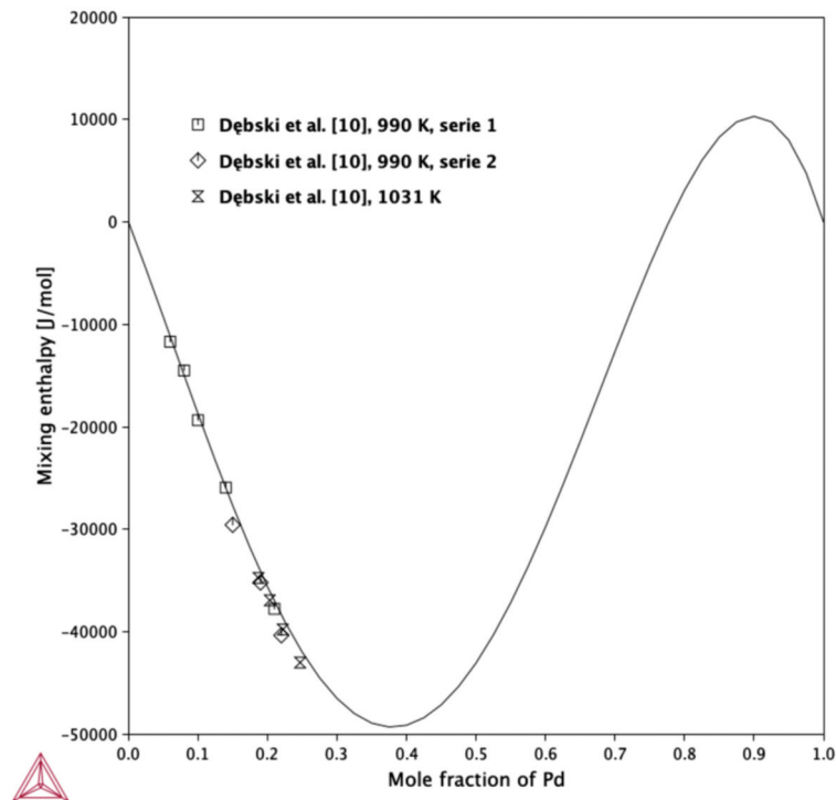
Figure 7. Calculated enthalpy of mixing of liquid Mg-Pd at 990 K superimposed with experimental data given by Dębski et al. [10] and obtained in this work
