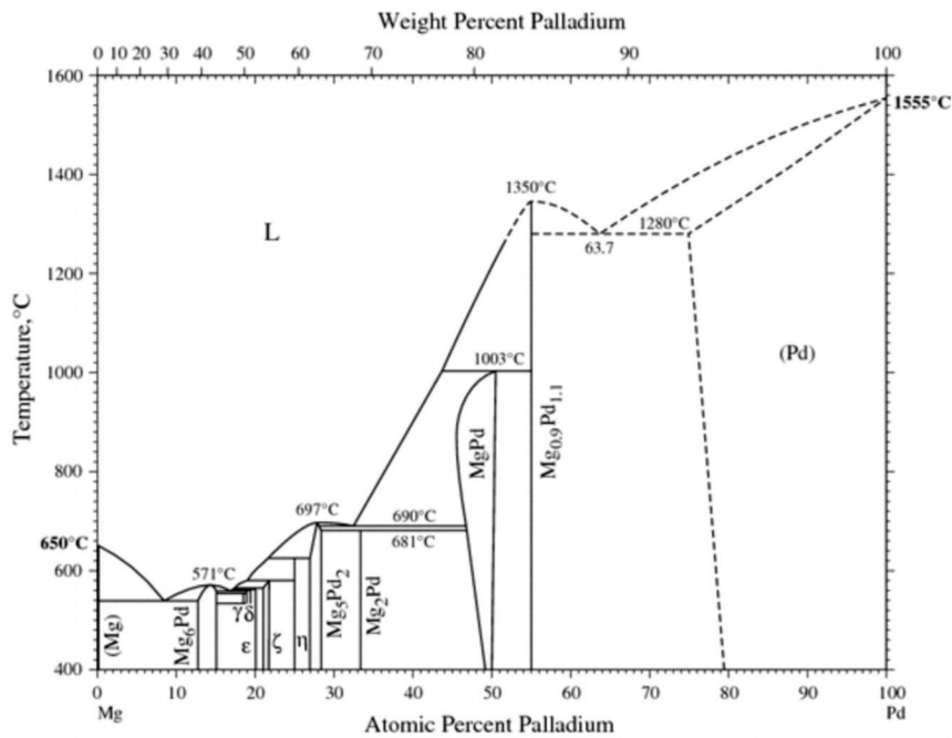
Figure 1b. A phase diagram of the Mg-Pd system proposed by Okamoto [7]
