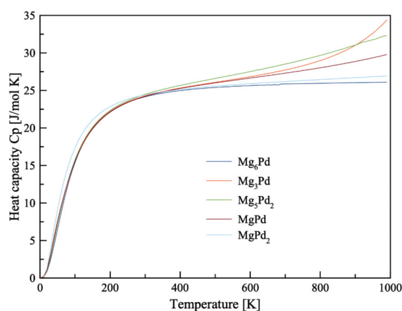
Figure 5. Calculated heat capacities of intermetallic compounds in the Mg-Pd system
