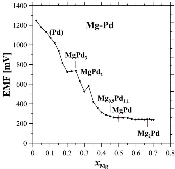
Figure 3. Coulometric titration curve for the Mg-Pd system for measurements made at 918 K
