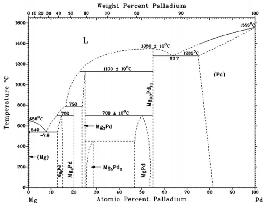
Figure 1a. A phase diagram of the Mg-Pd system proposed by Nayeb-Hashemi and Clark [1]
