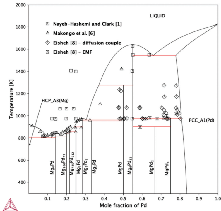
Figure 6. Calculated phase diagram superimposed with experimental data given by [1], [6], [8]
