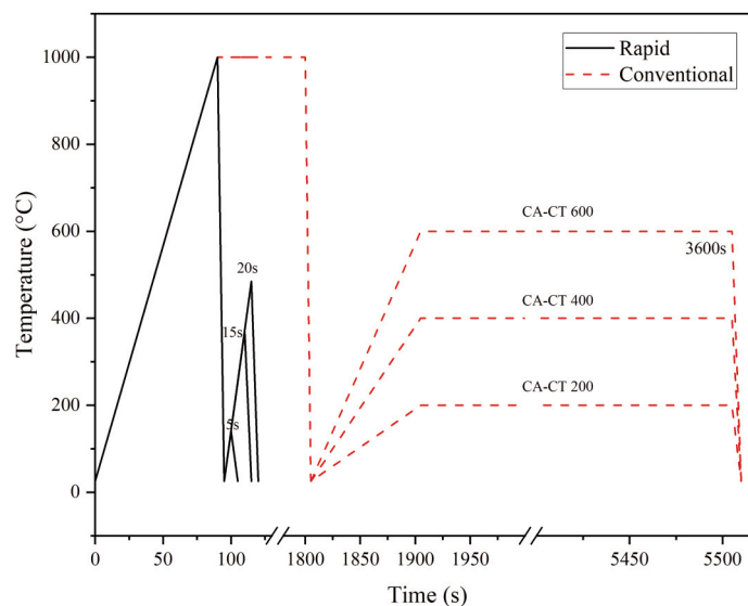
Figure 1. Schematic of the heat treatment parameters applied in this study
