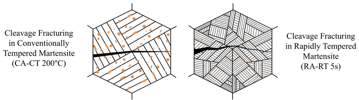
Figure 9. Schematic of crack propagation in the tempering treatment on CA-CT 200 °C (left) and RA-RT 5s (right) specimens
