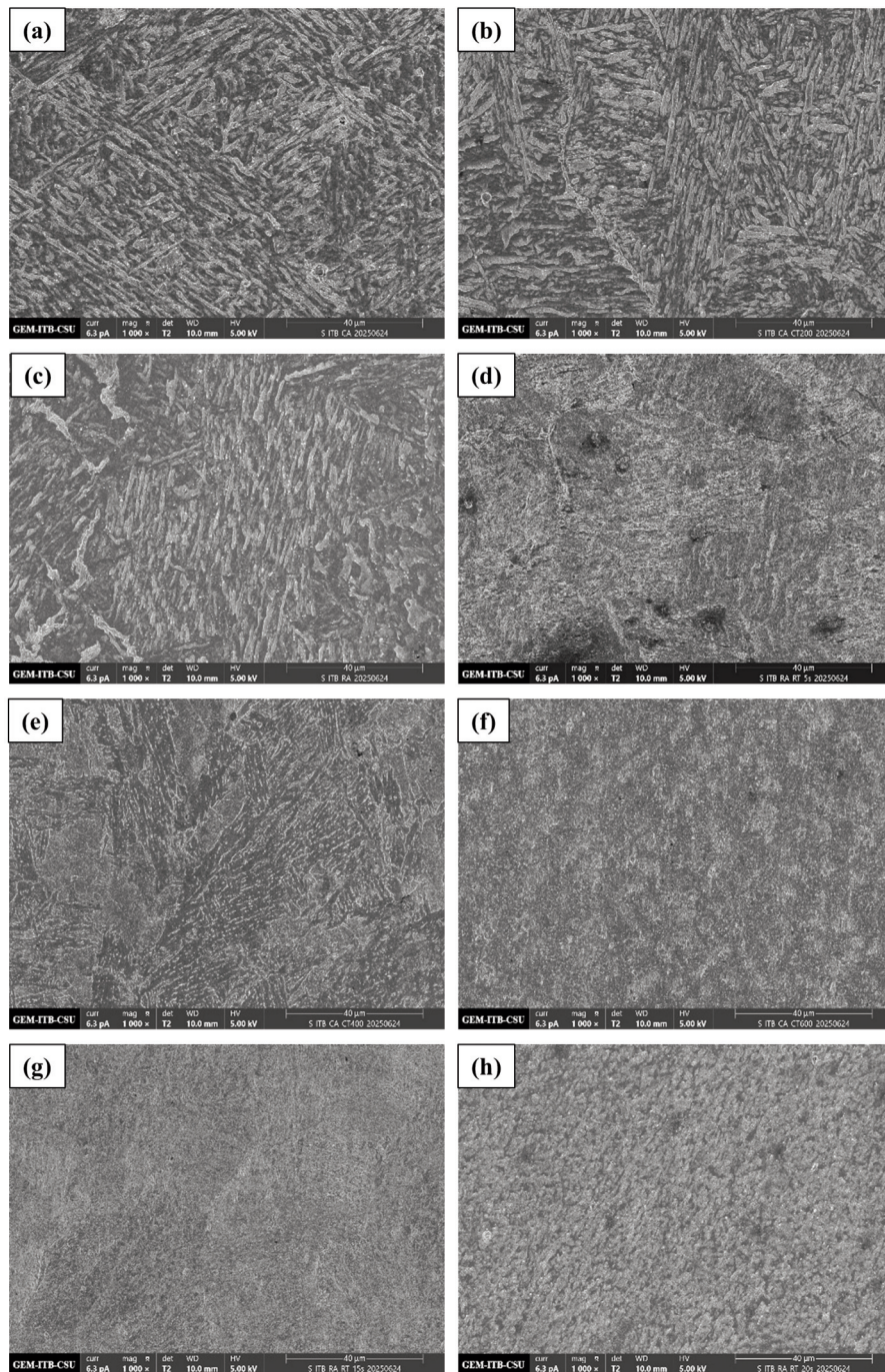
Figure 5. SEM-SE images showing the microstructures of specimens (a) CA, (b) RA, (c) CA-CT 200, (d) RA-RT 5s, (e) CA-CT 400, (f) RA-RT 15s, (g) CA-CT 600, and (h) RA-RT 20s, at 1.000× magnification
