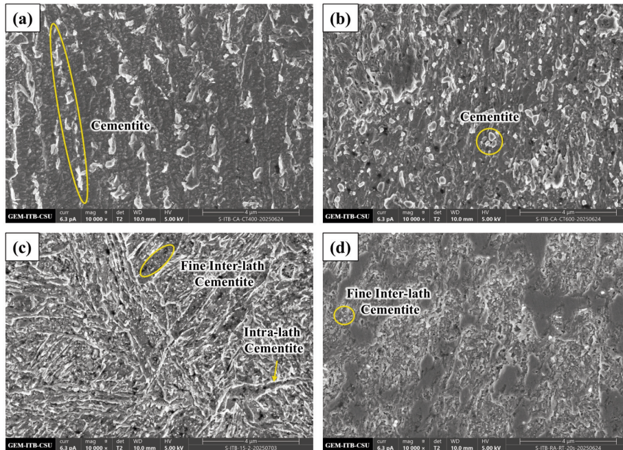
Figure 6. SEM-SE images showing the microstructures of specimens (a) CA-CT 400, (b) CA-CT 600, (c) RA-RT 15s, and (d) RA-RT 20s, at 10,000 \times magnification
