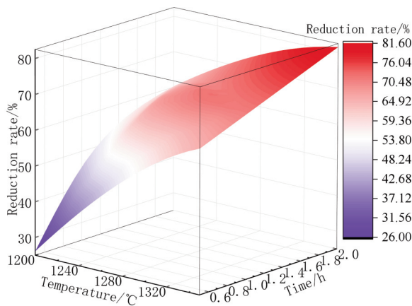
Figure 6. Effects of reduction temperature and reduction time on magnesium reduction rate
