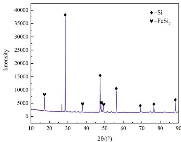
Figure 2. Phase analysis of ferrosilicon
