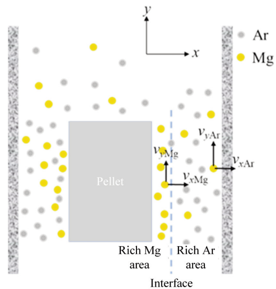
Figure 3. Schematic diagram of flowing argon atmosphere magnesium smelting theory
