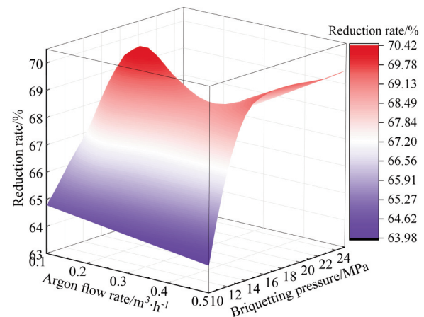
Figure 5. The influence of gas flow rate and briquetting pressure on magnesium reduction rate
