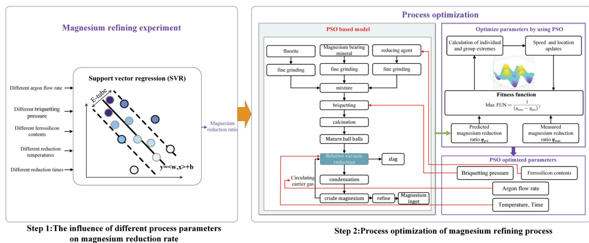
Figure 1. The flowchart of machine learning
