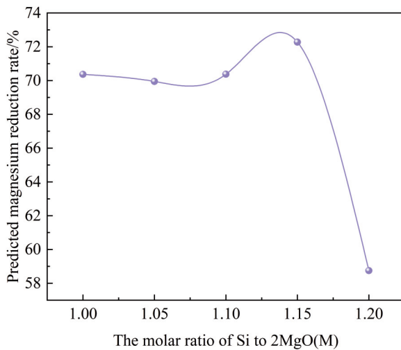
Figure 7. Effects of ferrosilicon content on magnesium reduction rate
