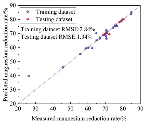
Figure 4. Comparison between predicted and measured magnesium reduction rate in training and testing datasets
