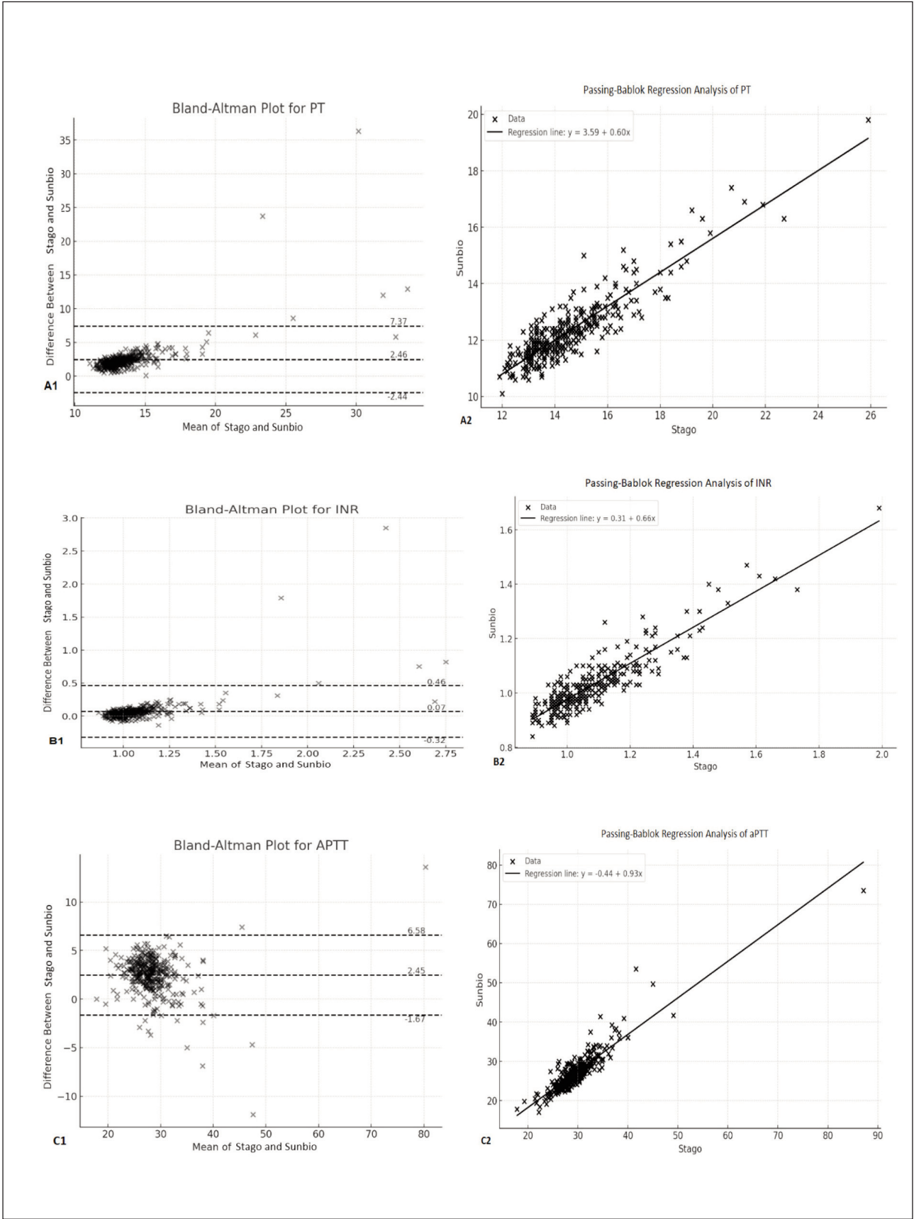
Figure 1 Comparison of tests by applying Bland-Altman plots and Passing-Bablok regression models. PT (A1, A2); INR (B1, B2); aPTT (C1, C2).
