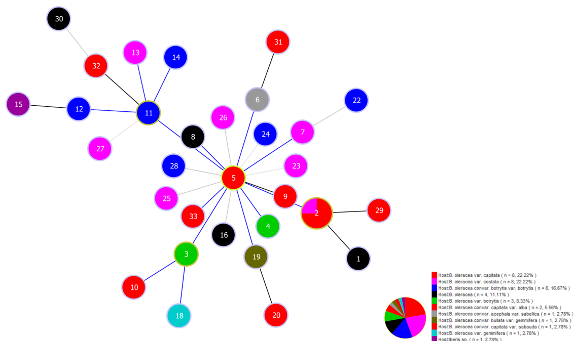
Figure 1. The MS tree showing distribution of 33 Xcc STs obtained for four genes ( P-X-dnaK , fyuA , gyrB , and rpoD ) in Serbian cabbage Xcc isolates and 33 comparative Xcc strains from different hosts and countries
