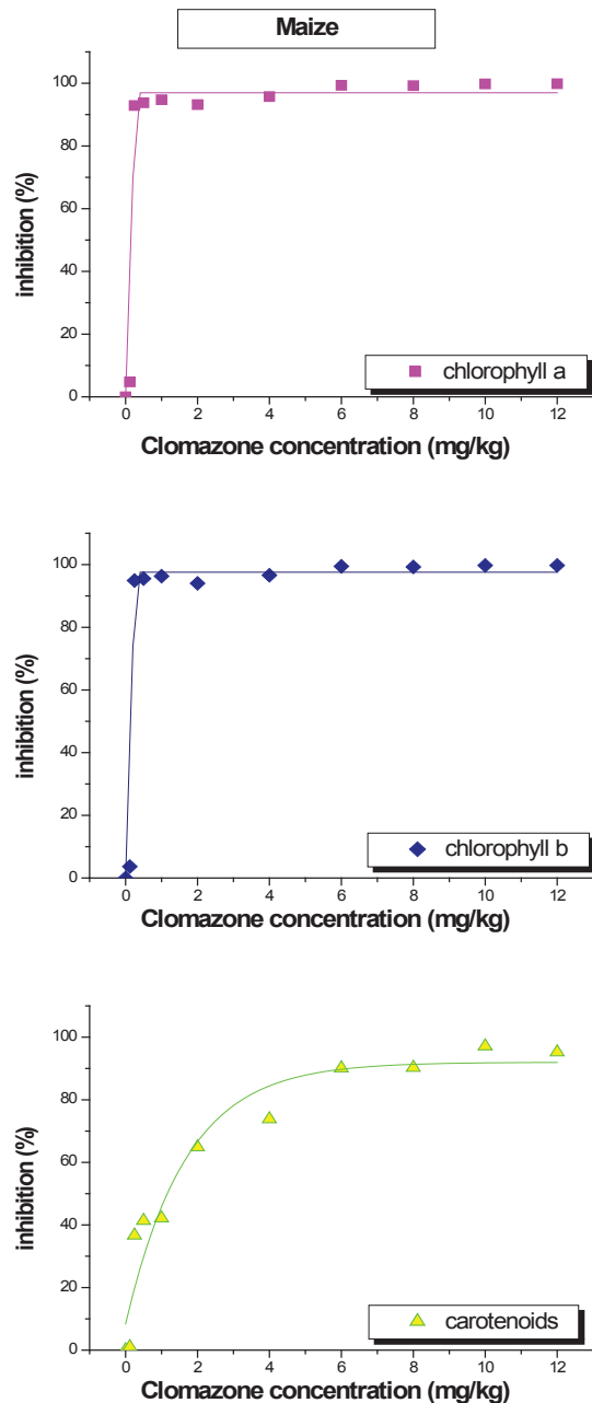
Figure 4. The residual effect of clomazone on chlorophyll a , chlorophyll b and carotenoids in leaves of maize
