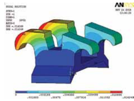
Figure 4. Deformed SS bracket (40° angle of twist).
