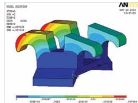
Figure 6. Comparison of slot (top) deformation in SS and ceramic brackets.
