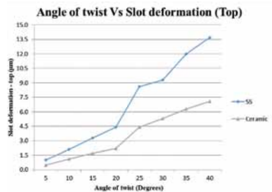
Figure 6. Comparison of slot (top) deformation in SS and ceramic brackets.
