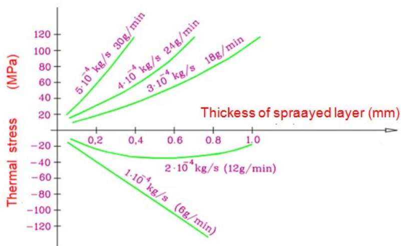
Figure 2 – Residual stresses in the ZrO_2.5CaO coating as a function of deposition speed
