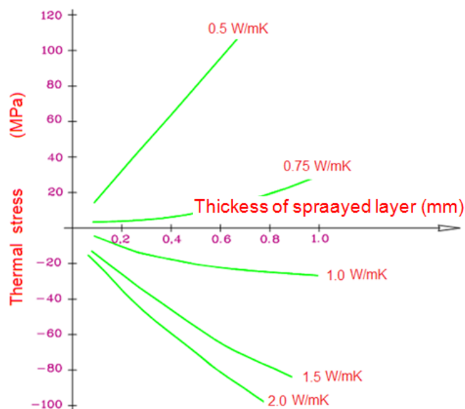
Figure 4 – Influence of thermal conductivity of residual stresses in the ZrO_2.5CaO coating
