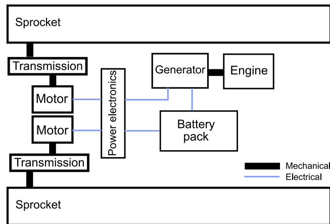
Figure 1 – Proposed powertrain configuration
